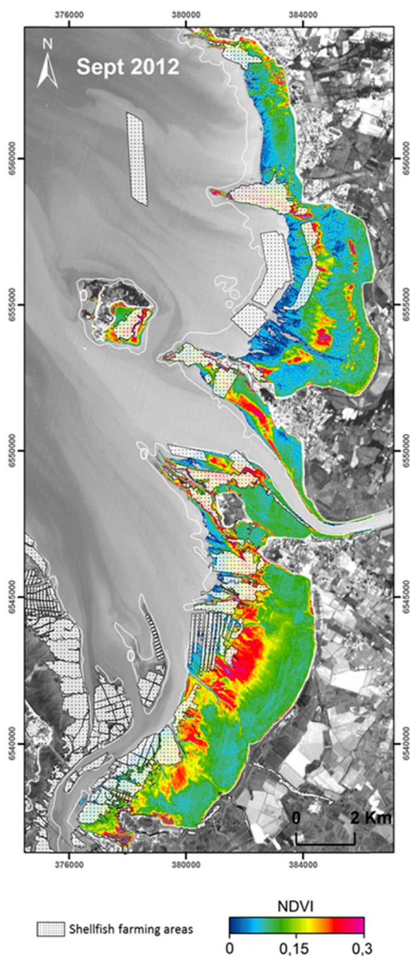
Fig. 6. Satellite remote sensing image of the eastern side of the Marennes-Oléron Bay in September 2012. Microphytobenthos is identified with a normalized difference vegetation index (NDVI), with a threshold between 0 and 0.3. Red color indicates the highest level of biomass. The dotted polygons represent shellfish farming areas. SPOT 5 satellite image with a spatial resolution of 20 m. (For interpretation of the references to color in this figure legend, the reader is referred to the Web version of this article.)
