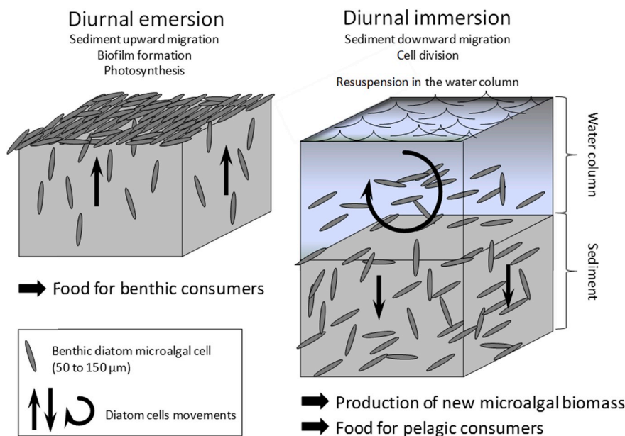
Fig. 4. Conceptual diagram of the processes leading to microphytobenthos primary production on intertidal bare mudflats in relation with the alternance of tides: Upward migration of diatoms during low tide and process of suspension of benthic diatoms in the water column at high tide (modified from Blanchard et al., 2006).
